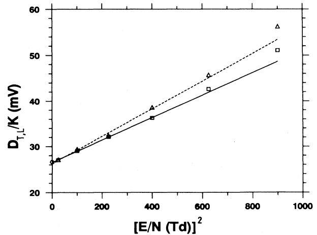
FIG. 6. Plots against (E/N)^2 of D_T/K for the present experimental data points (squares) and of D_L/K for the MCS (KMV) data points (triangles) showing their y intercepts for \text{Li}^+ in Kr. The theoretical limit value of 26.6 mV at 309 K is shown as a single hexagon on the y axis. The continuous and broken lines represent, respectively, the best-fit straight lines to the D_T/K and D_L/K data points for E/N \leq 20 Td.
