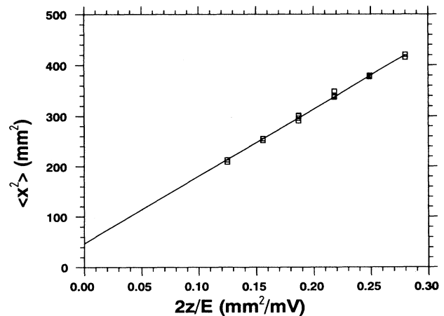
FIG. 3. The variance \langle x^2 \rangle plotted as a function of 2z/E for \text{Li}^+ ions in Kr at E/N=140 Td. The solid line represents the best-fit line which is extrapolated to 2z/E=0 to find the value of a_2 as given in Eq. (1).
